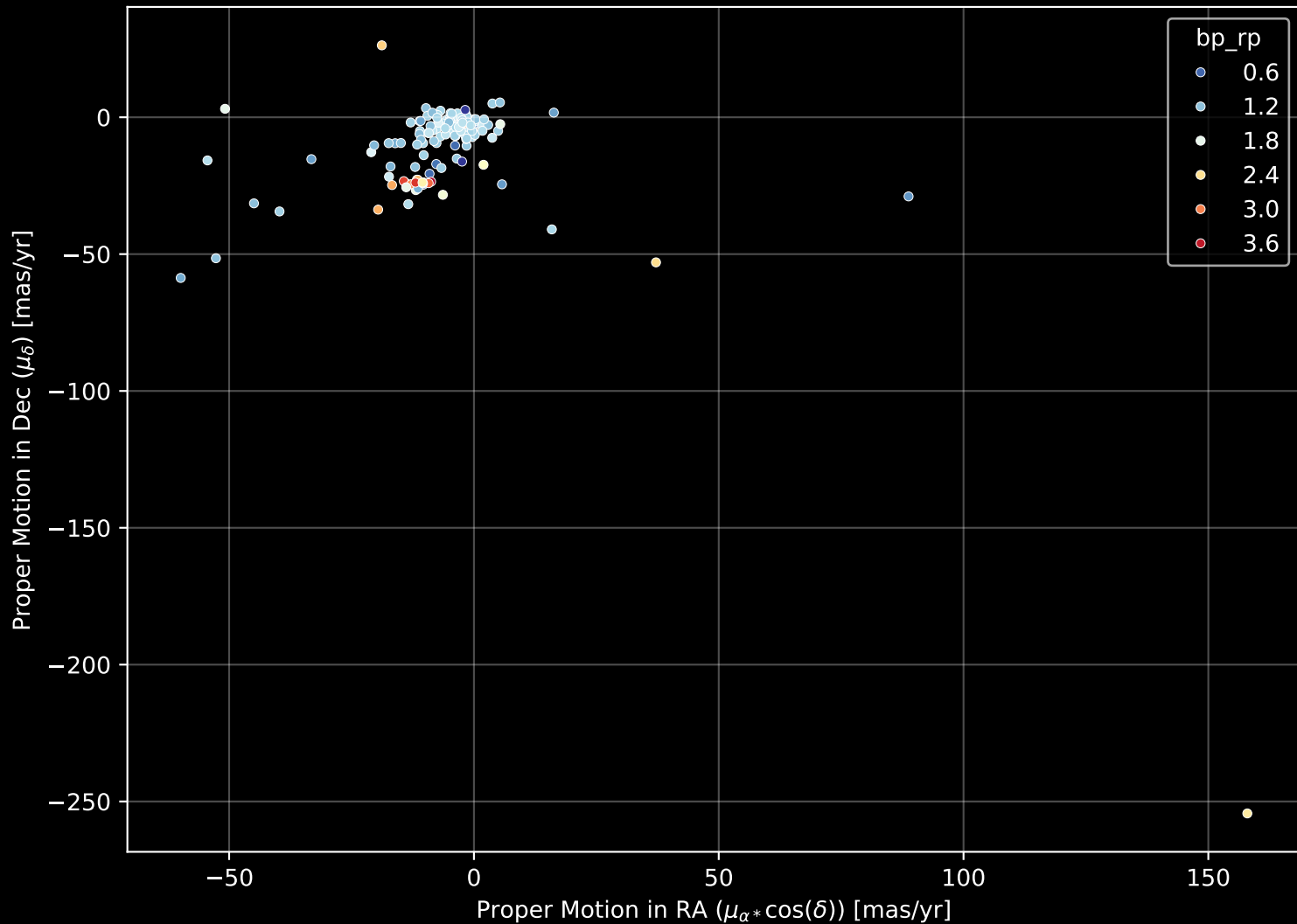
APOGEE DR17 Field: [350+20-O] Proper Motion Diagram (n= 143)
