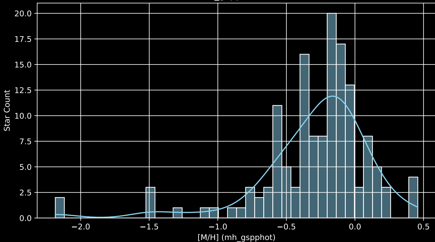
APOGEE DR17 Field: [350+20-O [M/H] (mh_gspphot) (n= 142)
