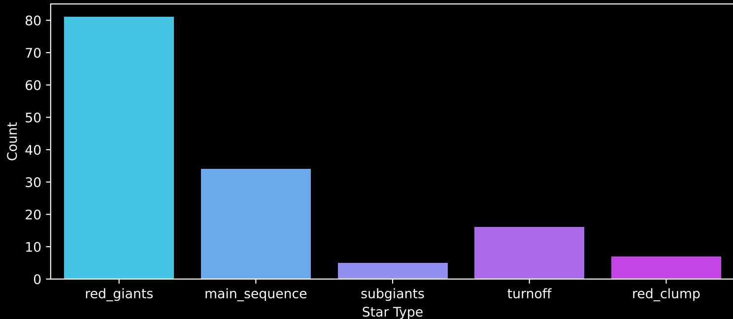
APOGEE DR17 Field: [350+20-O] Count plot of Star Type
