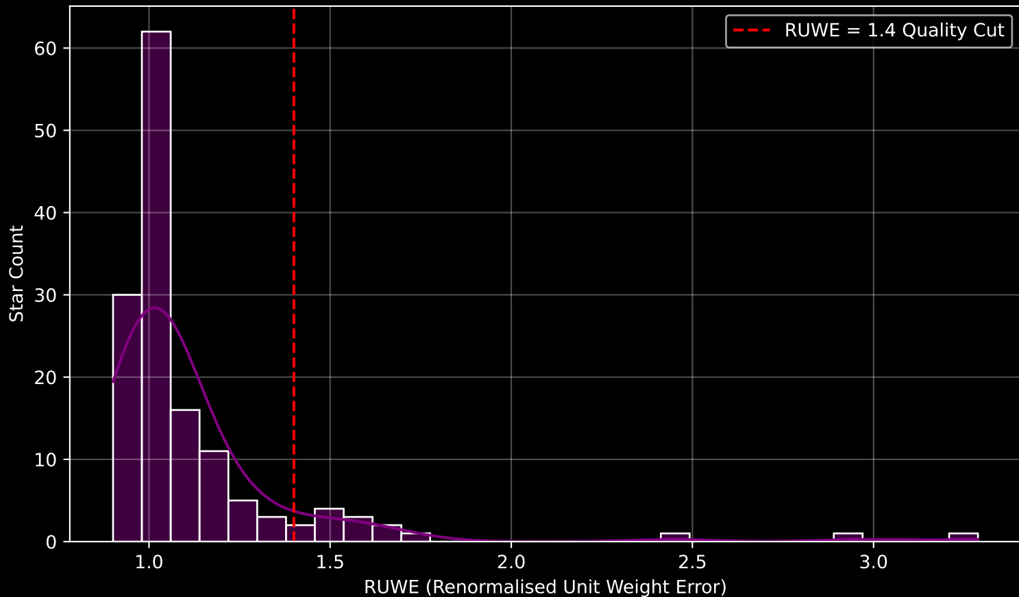
GAPOGEE DR17 Field [350+20-O] RUWE Distribution (n= 142)
