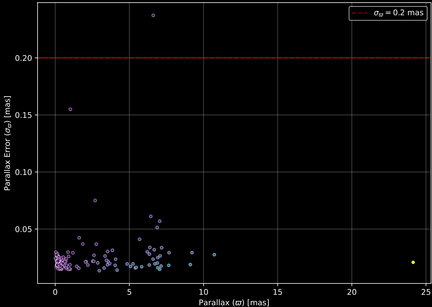
APOGEE DR17 Field: [350+20-O] Parallax Quality (n= 143)
