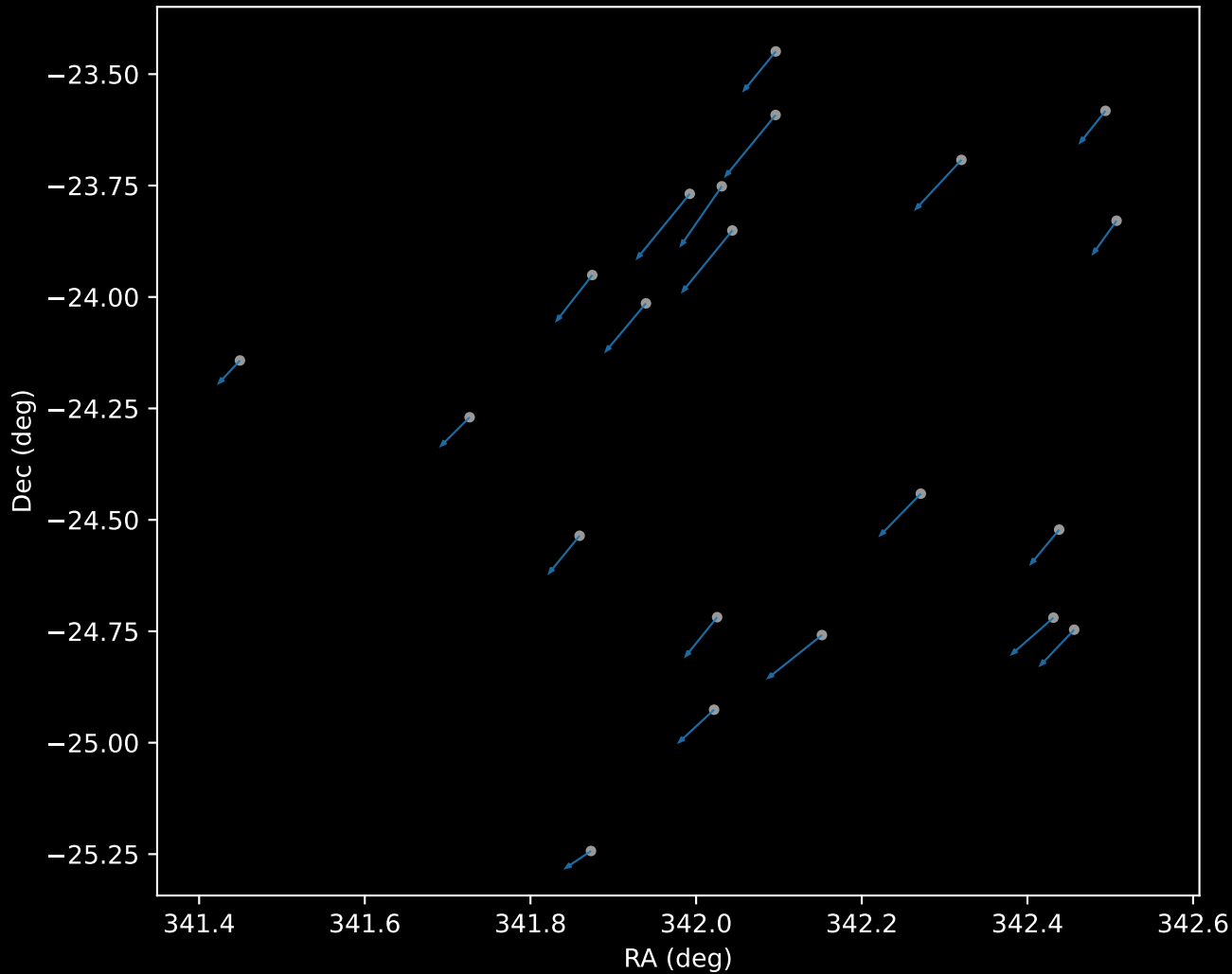
APOGEE DR17 Cluster 0 Proper Motion Vectors (n=21)
