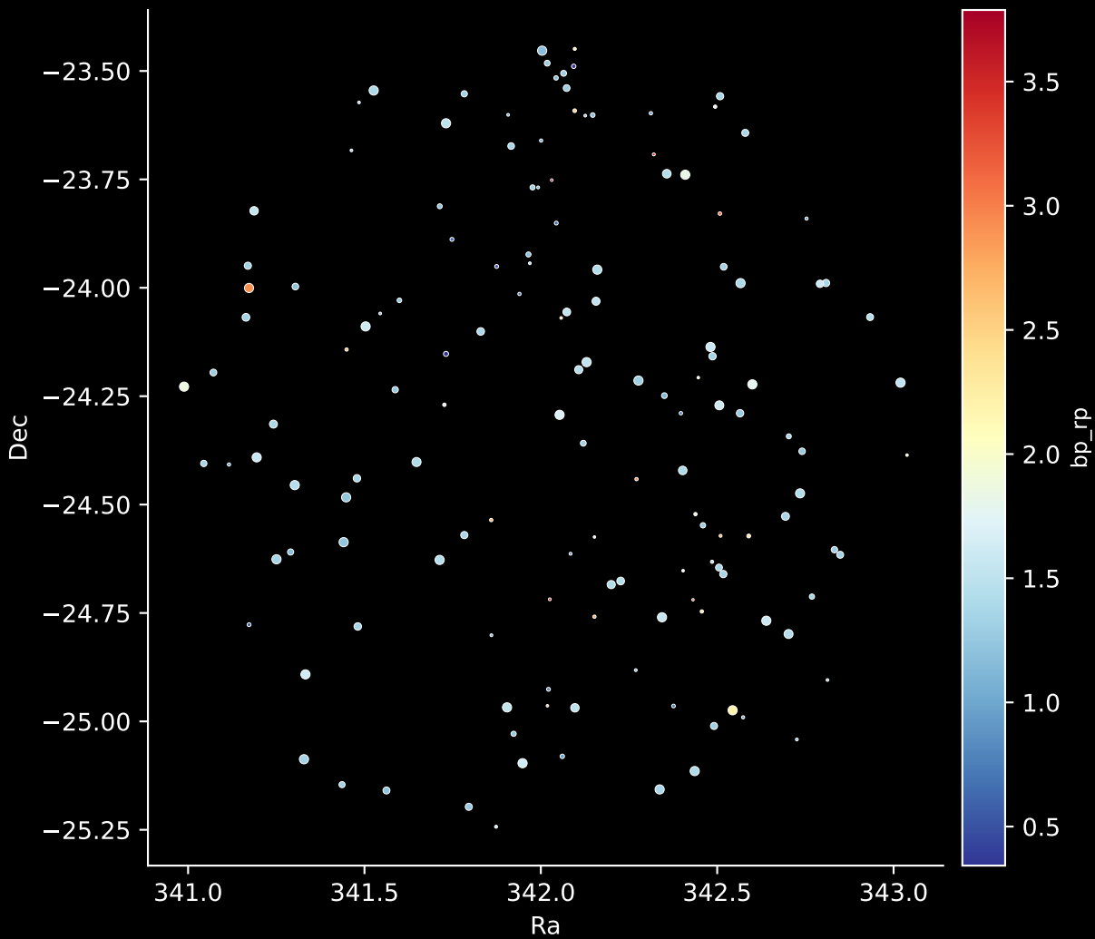
APOGEE DR17 Field: [350+20-O] Stars: 143
