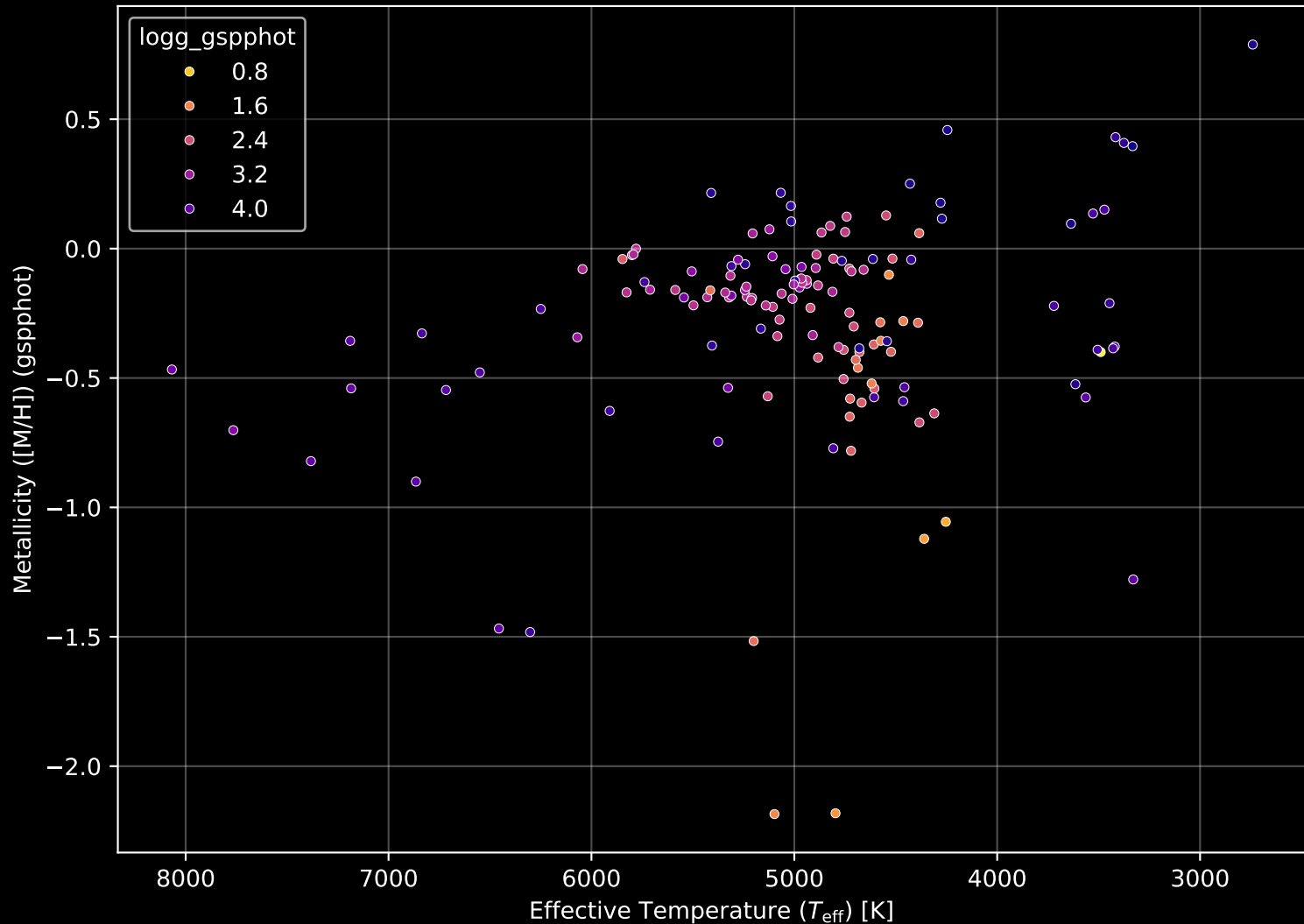
APOGEE DR17 Field: [350+20-O] Stellar Population Parameters (n= 143)
