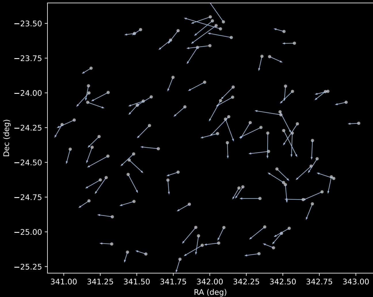
APOGEE DR17 Cluster 1 Proper Motion Vectors (n=96)
